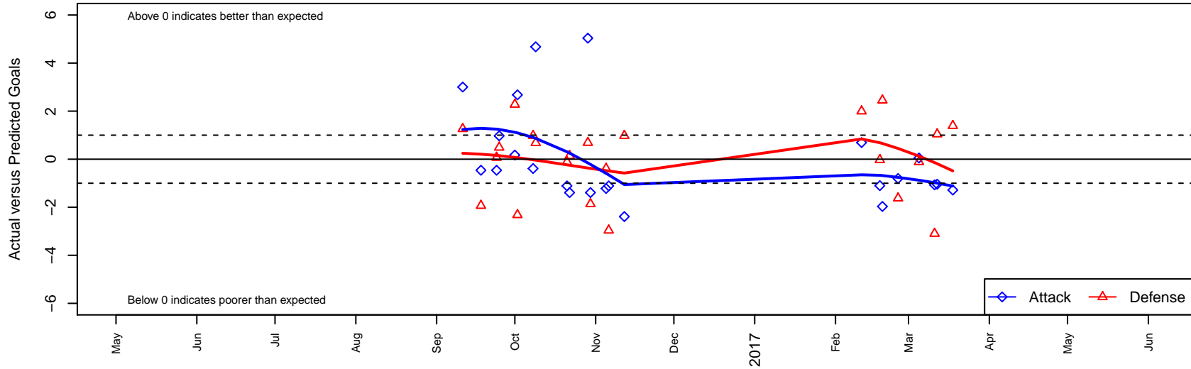
HSC Boca B05 Dots are actual minus expected GF (blue circles) and GA (red triangles). Blue line is smoothed change in attack strength. Red is smoothed change in defense strength.
